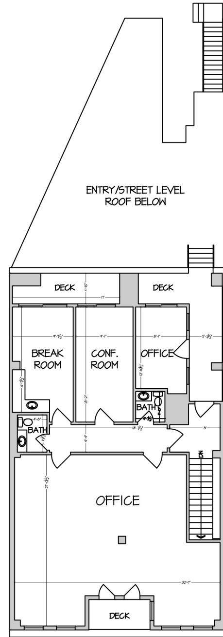
UPPER / 2ND LEVEL ±1,648 SQ. FT.
