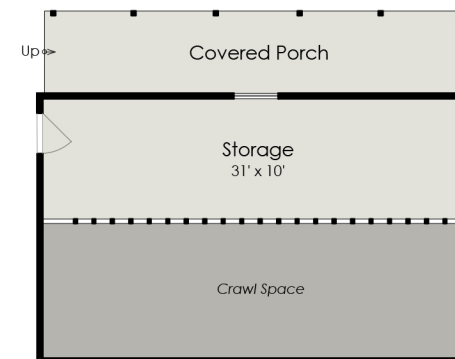
LOWER LEVEL 2
