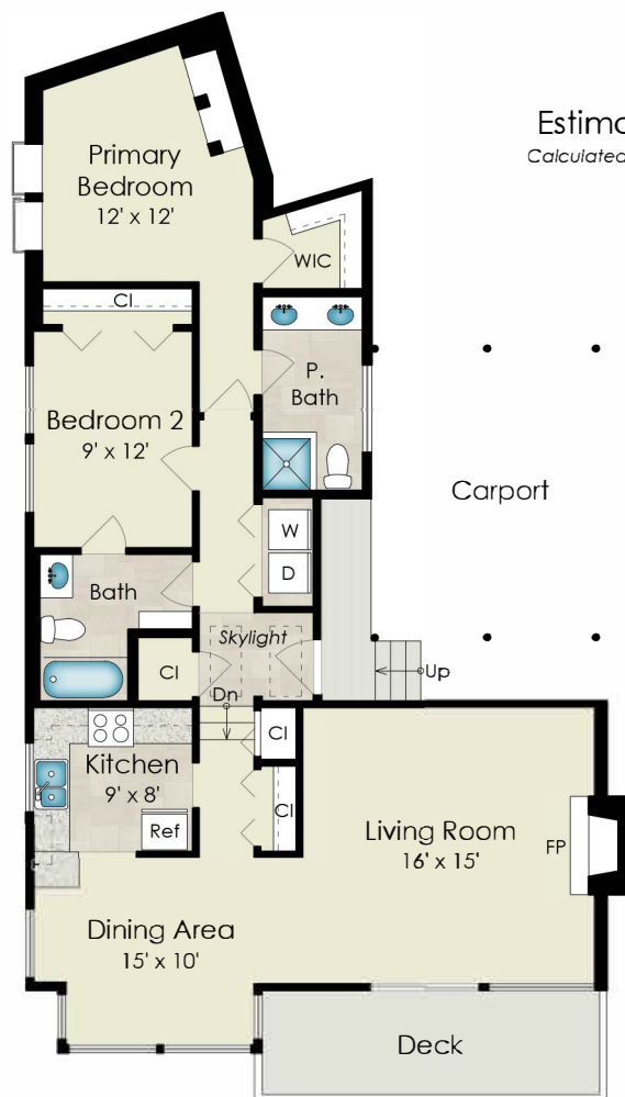
FLOOR PLAN
