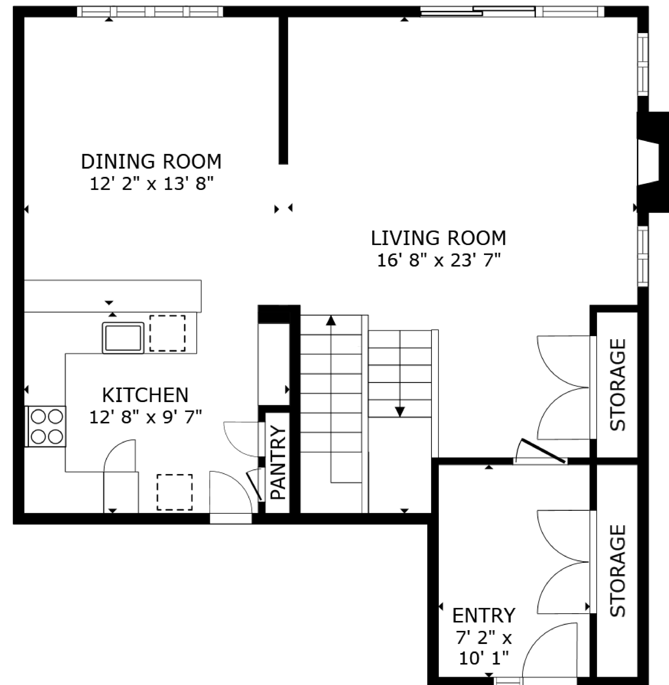
FLOOR 2
