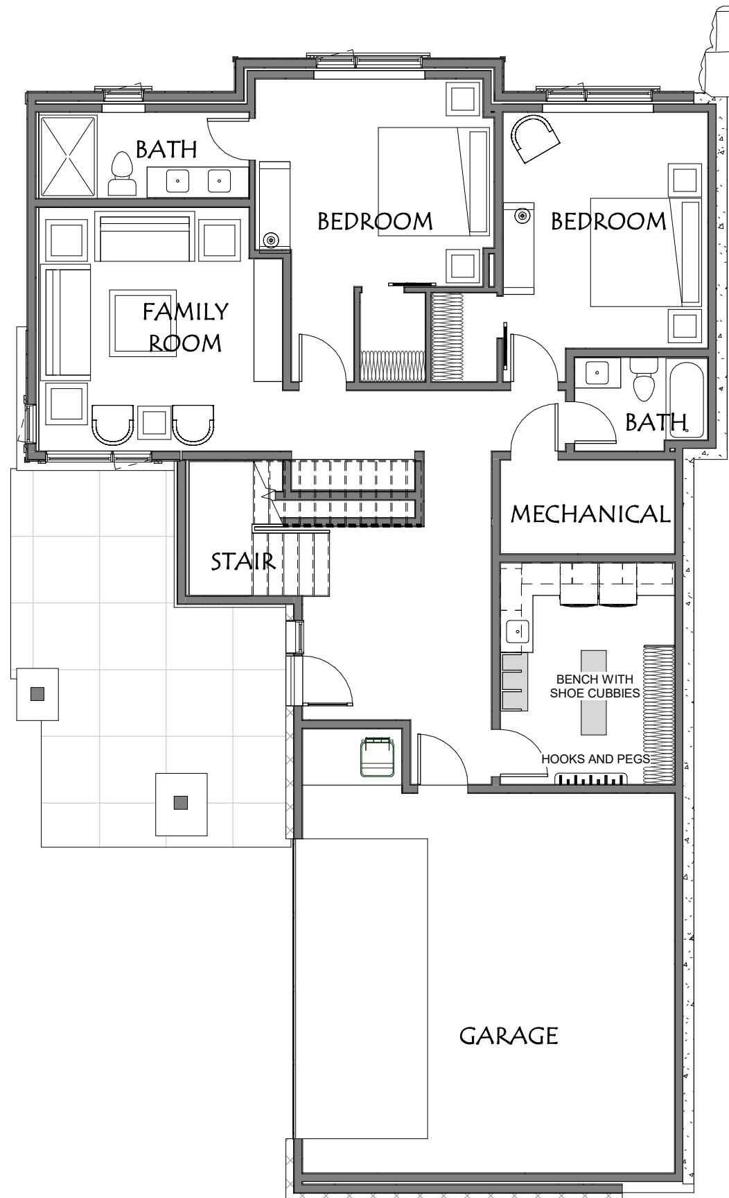
1 LOWER LEVEL - EAST UNIT 1/8" = 1'-0"
