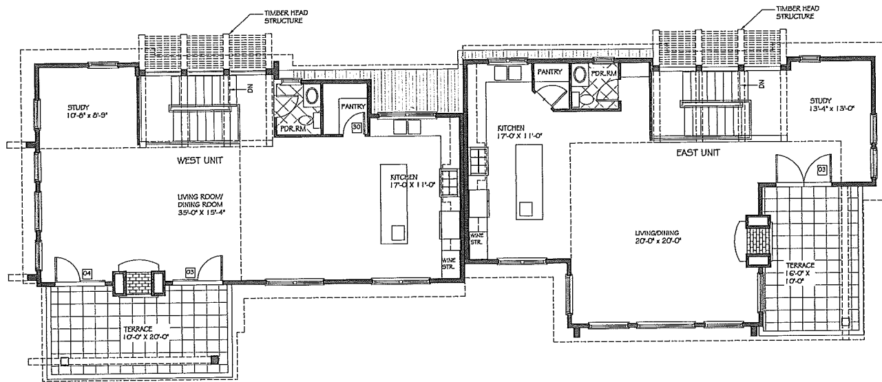
LIVING LEVEL PLAN 1/4" = 1'-0"
