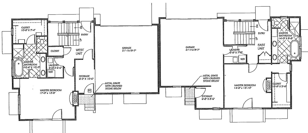
ENTRY LEVEL PLAN 1/4" = 1'-0"
