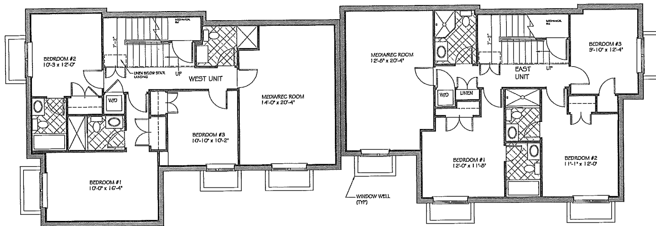
BEDROOM LEVEL PLAN 1/4" = 1'-0"
