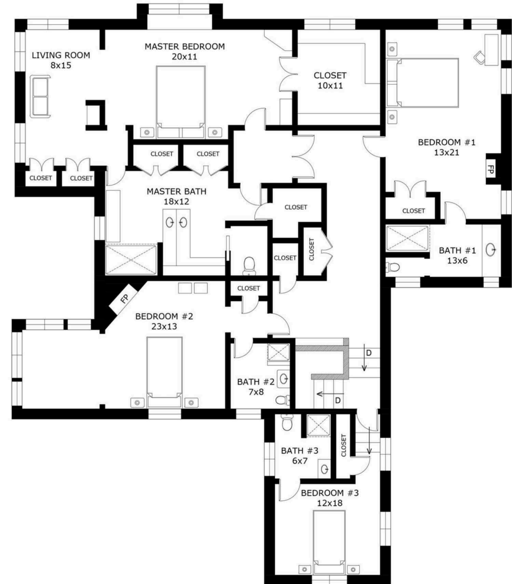
SECOND FLOOR
