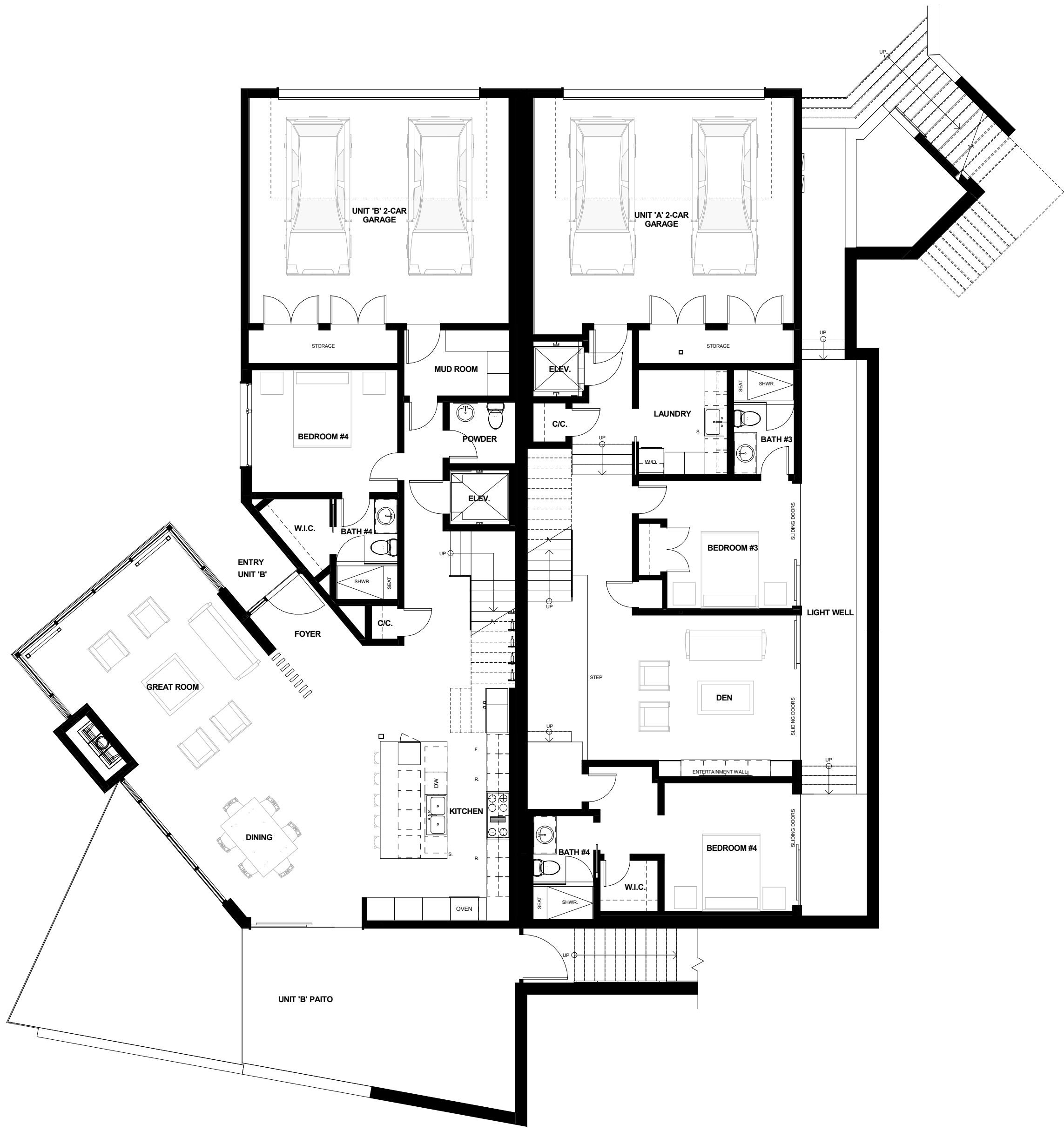
FIRST LEVEL FLOOR PLAN 2212 VERMONT COURT, VAIL, CO
